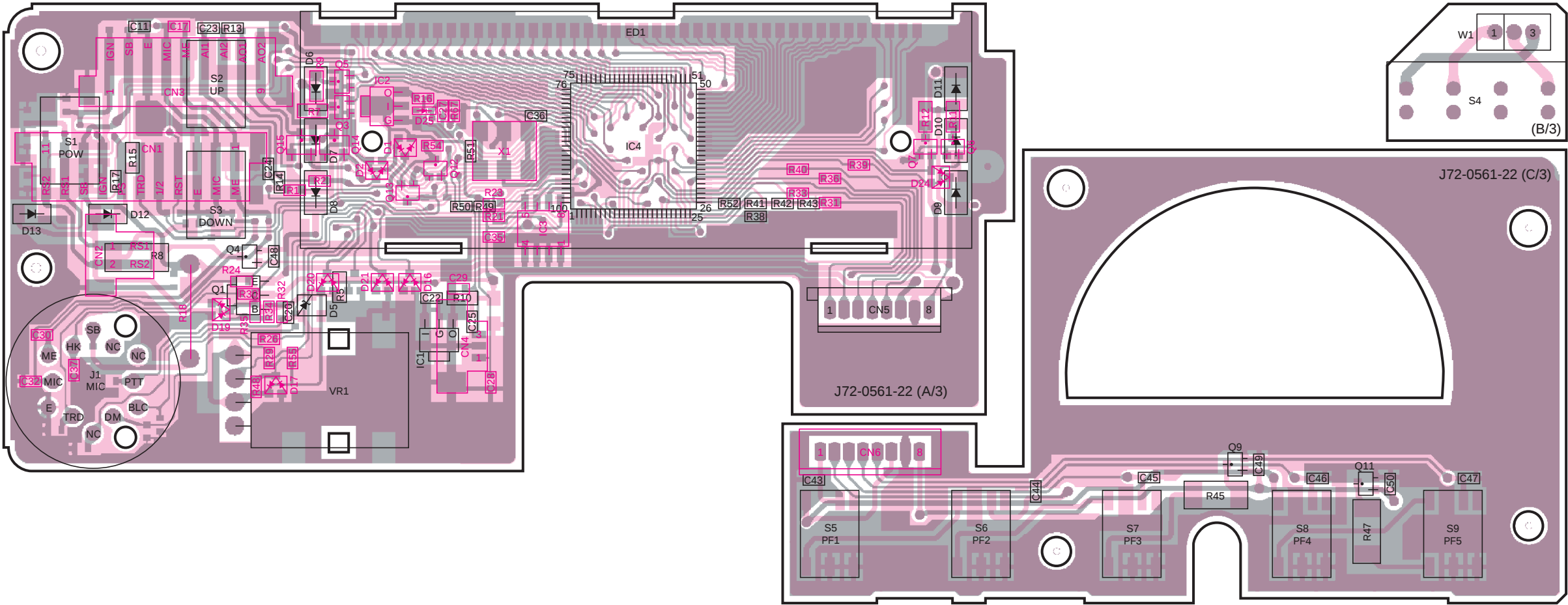
DISPLAY UNIT (X54-3190-20) Component side view : KCH-10
