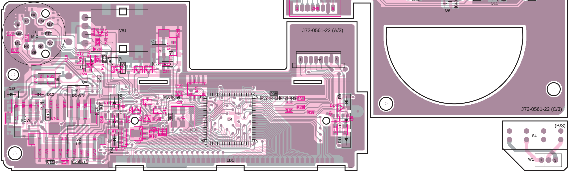
DISPLAY UNIT (X54-3190-20) Foil side view : KCH-10
