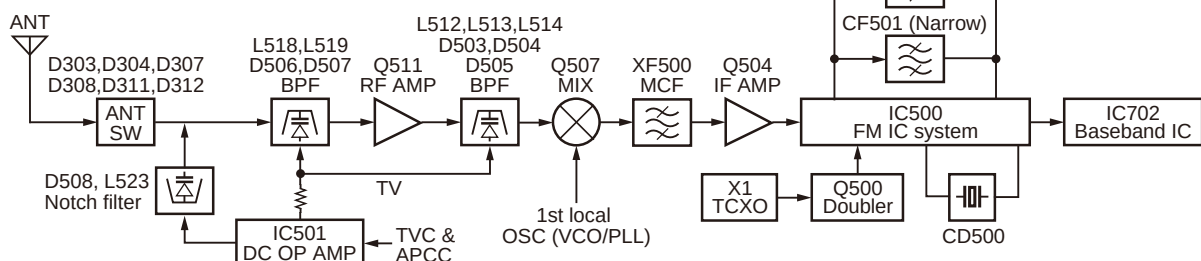
Fig. 2 Receiver System
