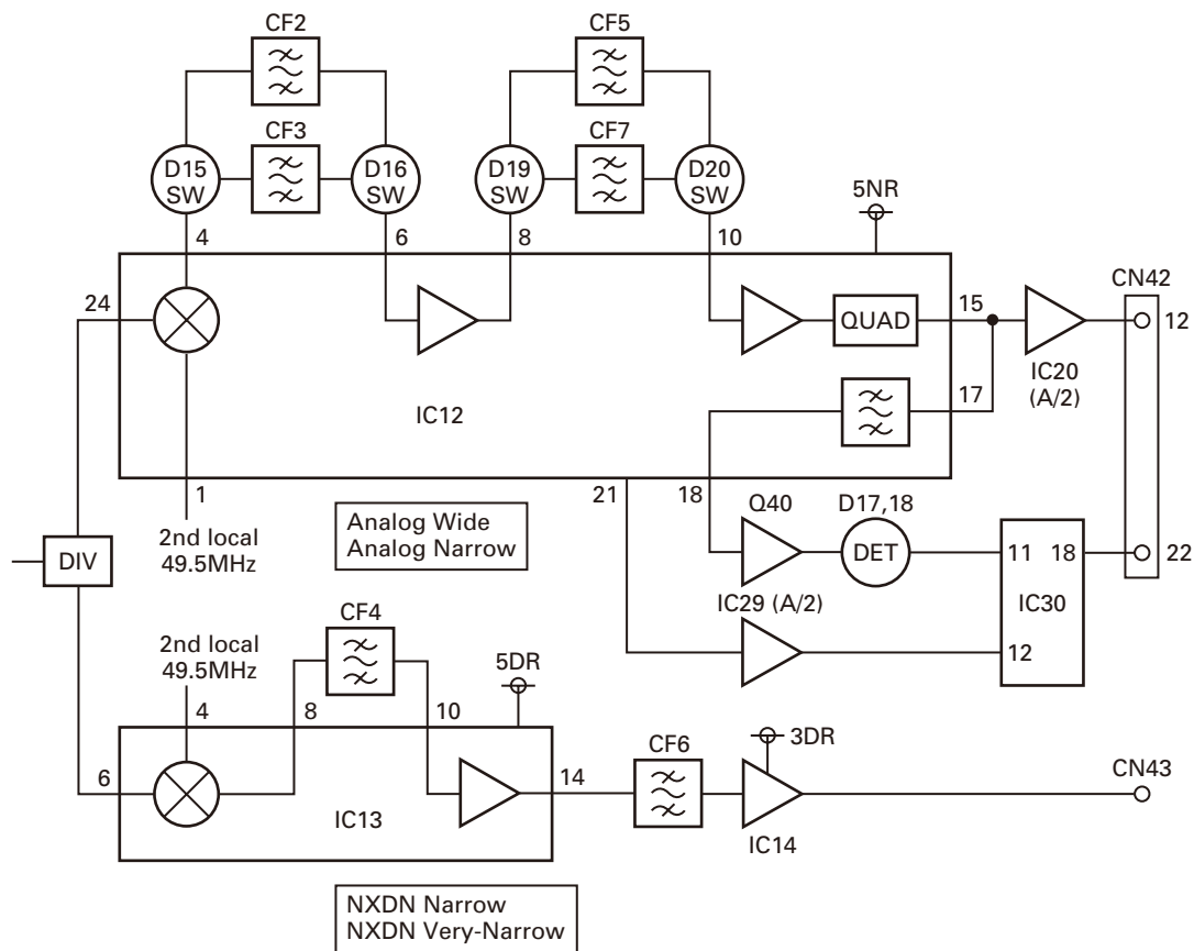
Fig. 19 Demodulator circuits
