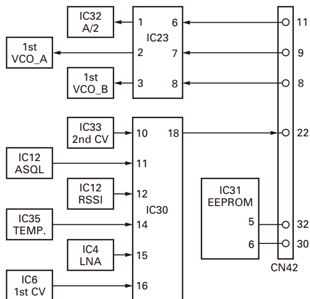
Fig. 23 Other circuits
