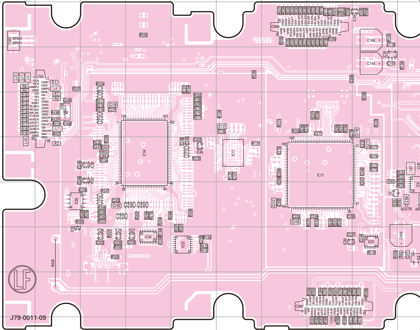
CONTROL UNIT (X53-4130-10) Component side view (J79-0011-09)
