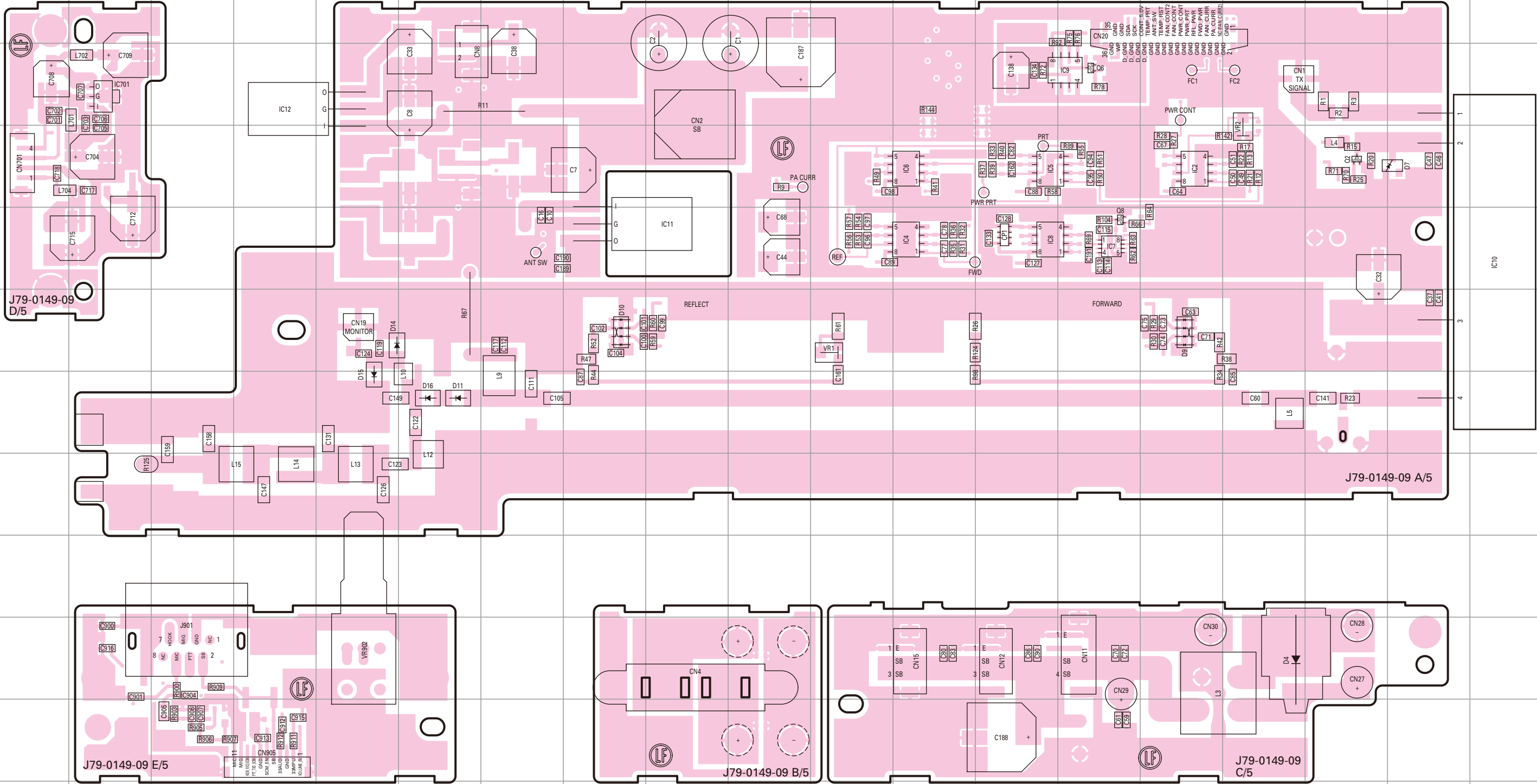
FINAL UNIT (X45-3820-10) Component side view (J79-0149-09)
