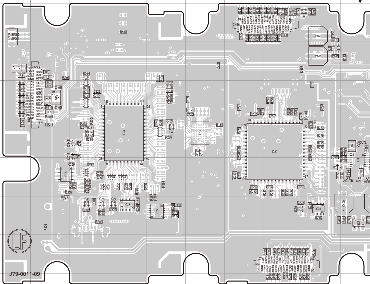
CONTROL UNIT (X53-4130-10) Component side view (J79-0011-09)
